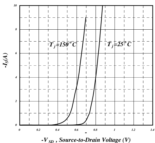
Reverse Diode
